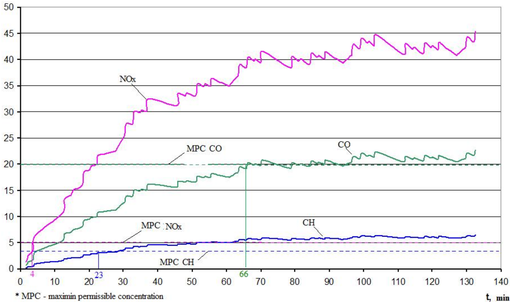
Concentration of NO x , CO & CH nearby working zone of track-laying trains.
